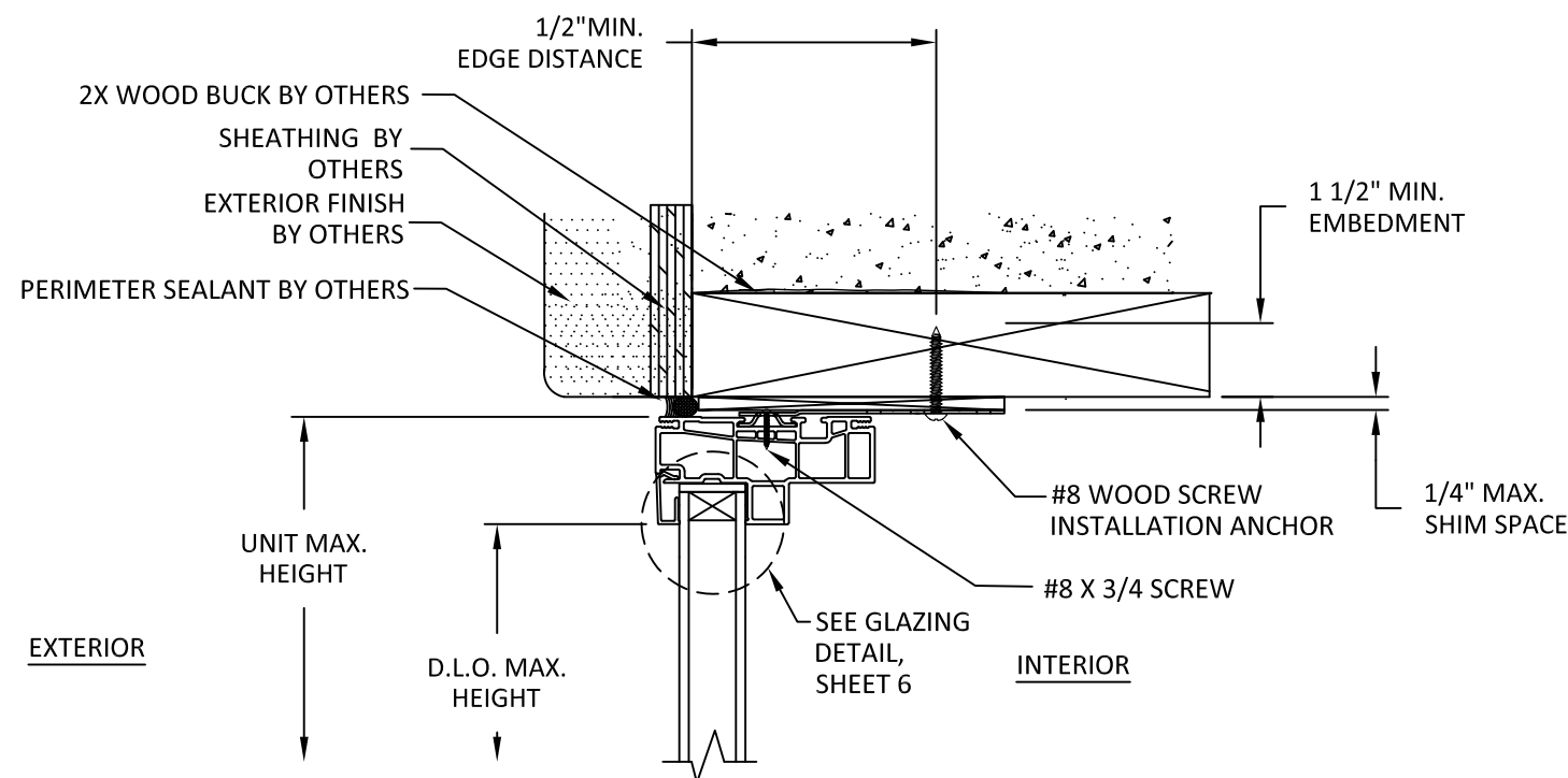
A 6 VERTICAL SECTION CLIP INSTALLATION WOOD SUBSTRATE
